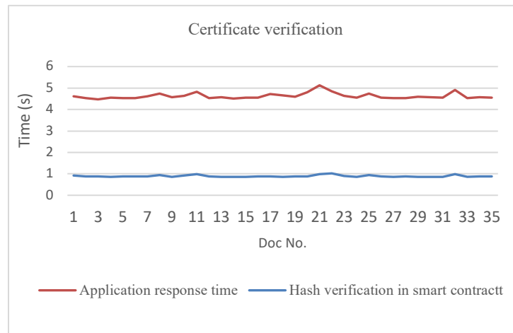
Figure 8 Response time for certificate verification
