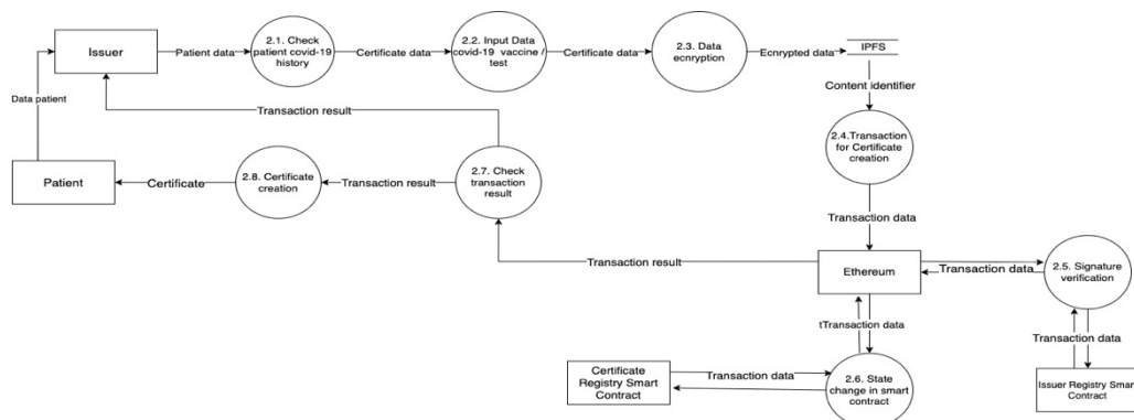
Figure 5 Data flow diagram of certificate creation
