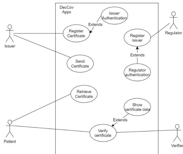
Figure 1 Use case diagram Covid-19 certificate storage system
