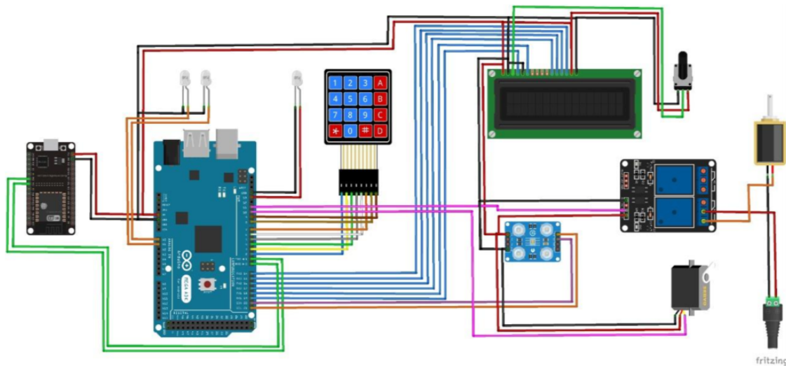
Figure 4. Hardware Design
