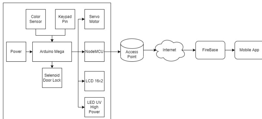
Figure 3. Block Diagram
