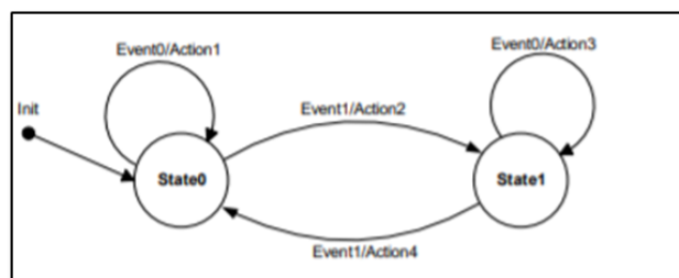
Figure 4. Simple State Diagram
