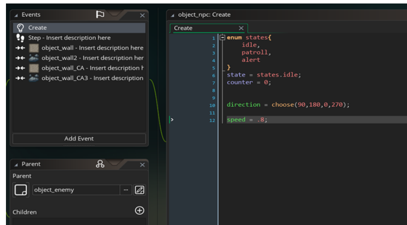
Figure 7. Source Code NPC
