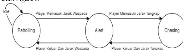
Figure 5. State chart of NPC Behavior in the Maze Game.
