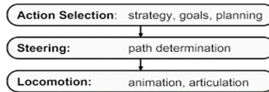
Figure 3. Movement Hierarchy of NPC Behavior
