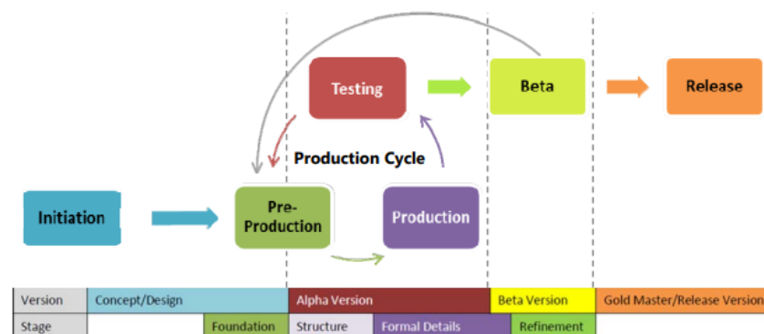
Figure 1. Game Development Life Cycle [7]
