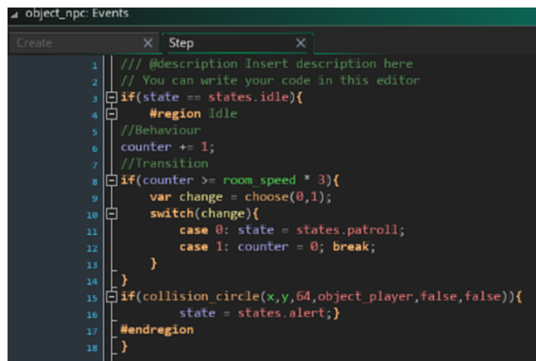
Figure 8. Source Code NPC
