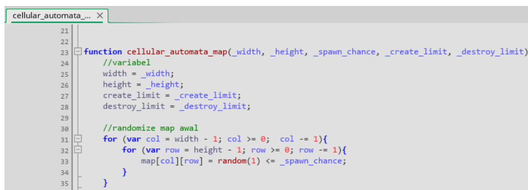
Figure 7. Source code of Cellular automata script
