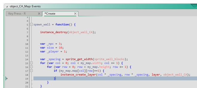
Figure 6. Source code for wall spawn
