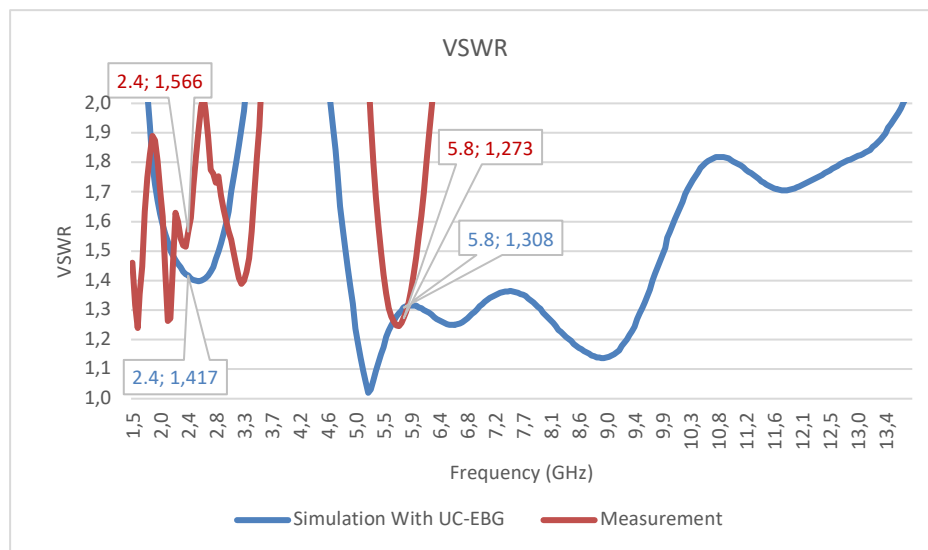
Figure 11. VSWR Results
