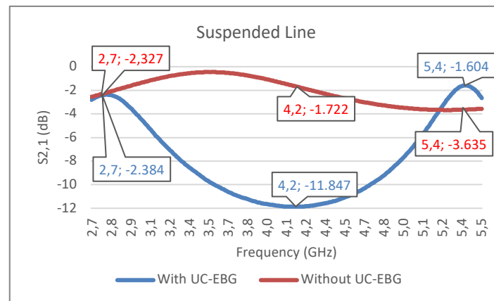
Figure 8. Comparison of Suspended Line Method Simulation Results
