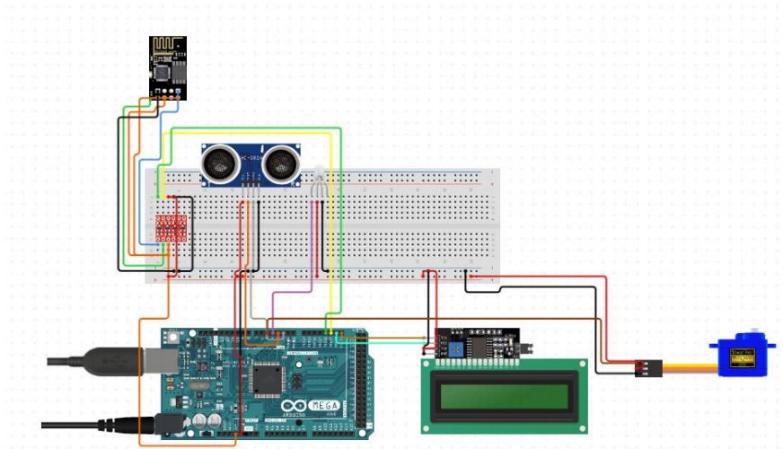
Figure 4. Hardware design
