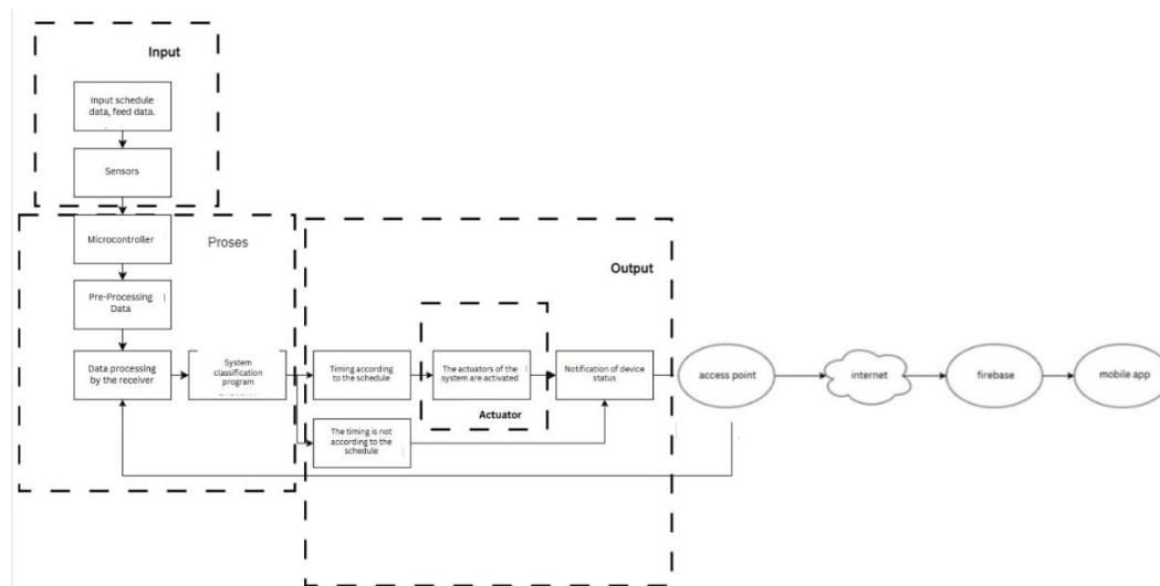
Figure 3. Block diagram
