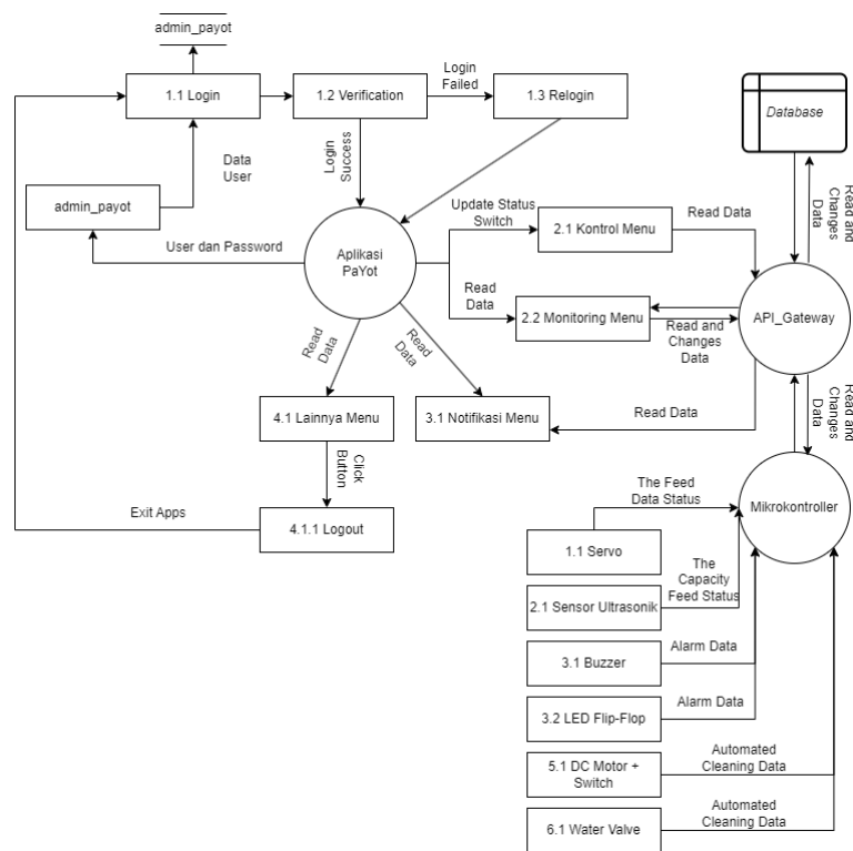
Figure 3. PaYot data flow diagram
