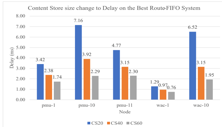
Fig. 8. Graph of Content Store size change to Delay on the Best Route-FIFO system.
