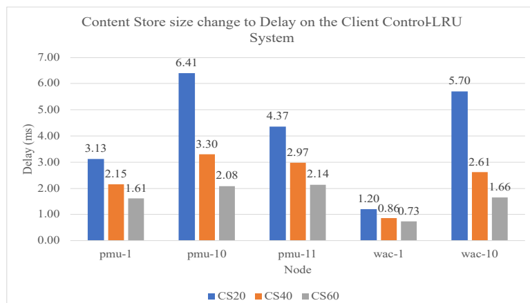
Fig. 9. Graph of changes in the size of the Content Store to the Delay of the Client Control-LRU system
