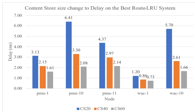
Fig. 7. Graph of Content Store size change to Delay on the Best Route-LRU system.
