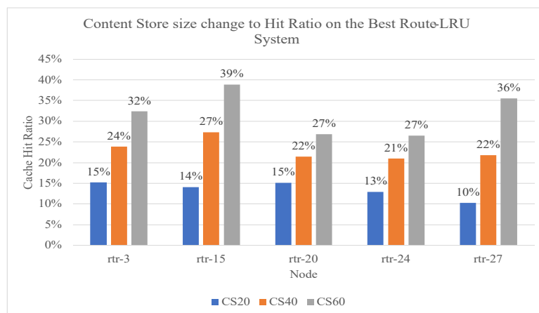
Fig. 3. Graph of changes in the size of the Content Store to the Hit Ratio on the Best Route-LRU system
