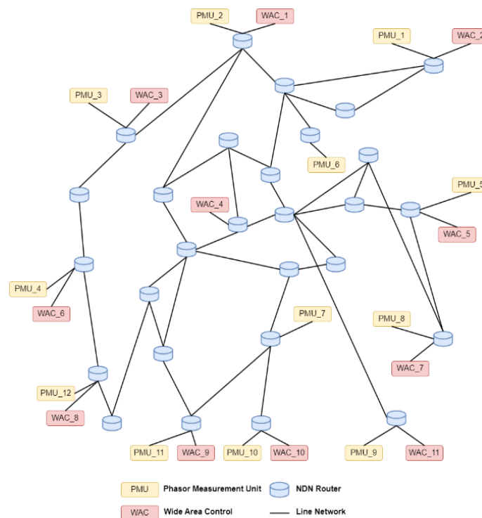
Fig. 1. NDN Smart Grid Topology
