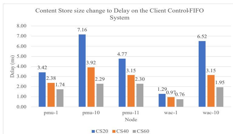
Fig. 10. Graph of Content Store size change to Delay on the Client Control-FIFO system
