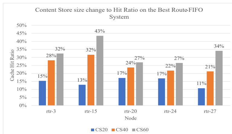
Fig. 4. Graph of changes in the size of the Content Store to the Hit Ratio on the Best Route-FIFO system
