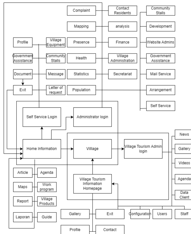
Figure 7. Activity Diagram Block Site
