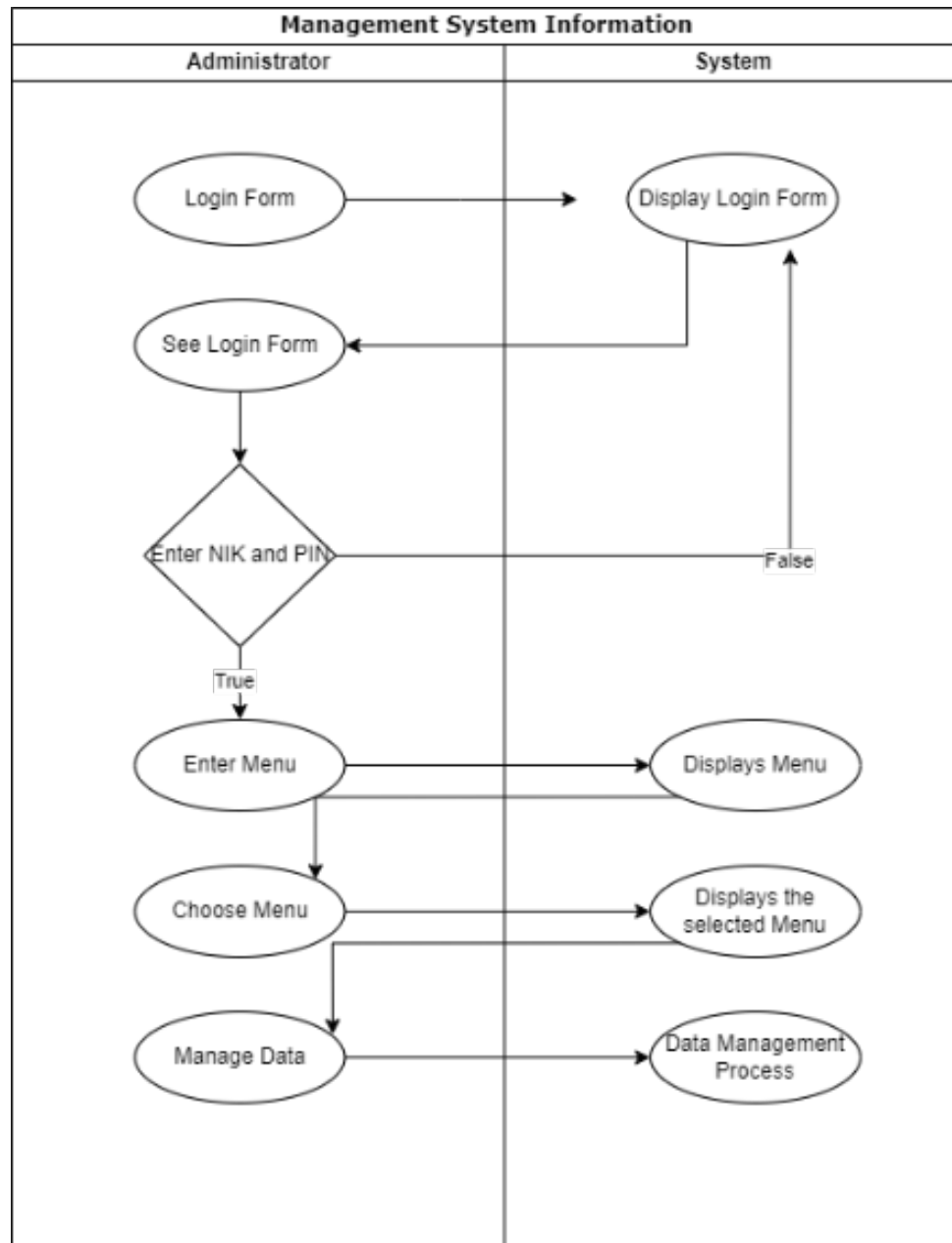
Figure 6. Activity Diagram Admin
