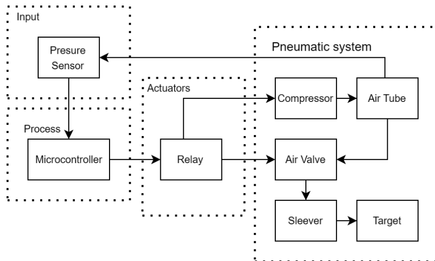
Figure 2. Block diagram system
