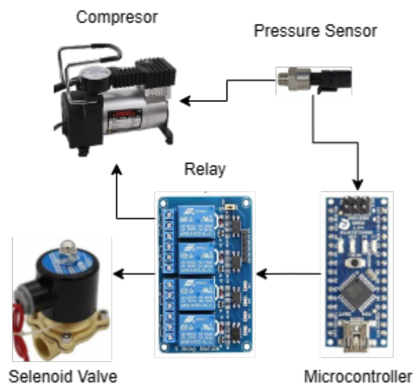
Figure 3. Hardware design
