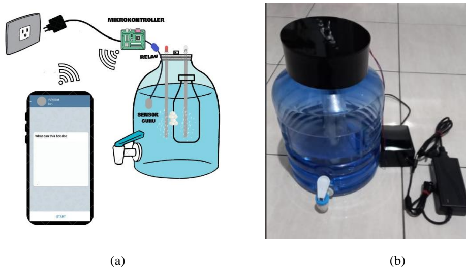
Figure 6. (a) System Design Mockup, (b) Final Result PWI System that has an Automatic Socket
