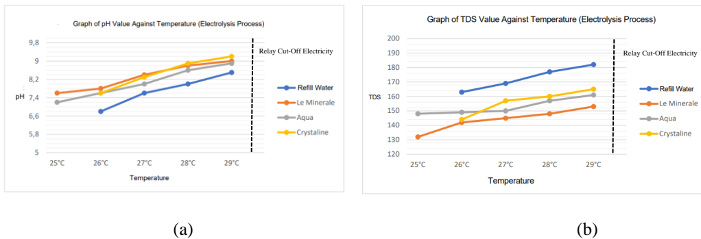
Figure 5. (a) Graph of pH value Against Temperature, (b) Graph of TDS value Against Temperature
