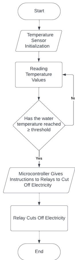
Figure 1. Electric current control system currentchart
