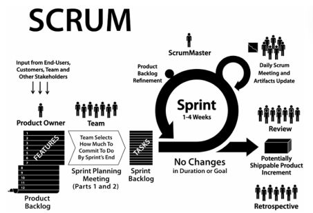
Gambar 1. Metode Scrum
