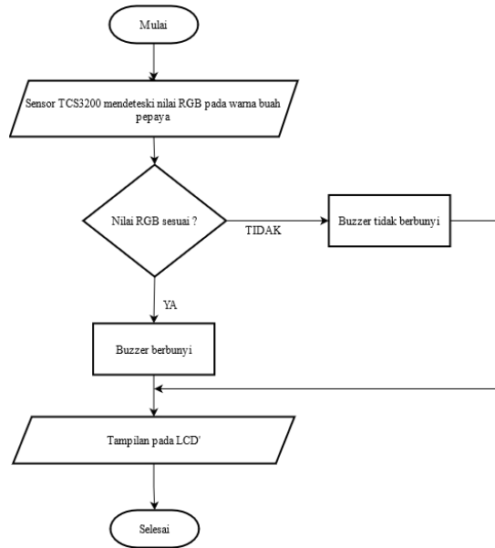
Gambar 3. Flowchart Program
