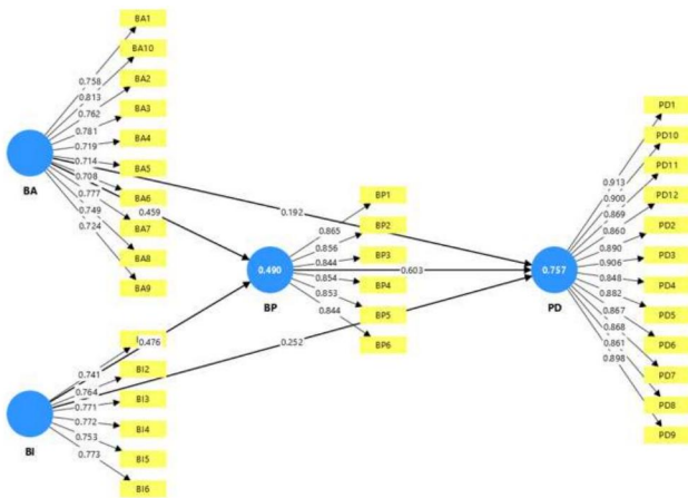
Gambar 4. Path Diagram Outer Model
