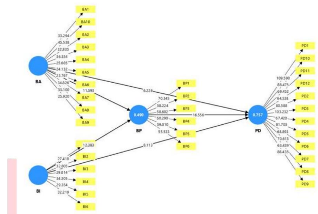
Gambar 5. Path Diagram Inner Model
