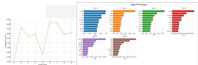
Gambar 6. Topic Modeling Responsiveness
