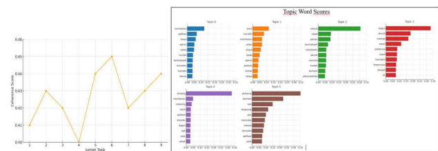
Gambar 5. Topic Modeling Reliability
