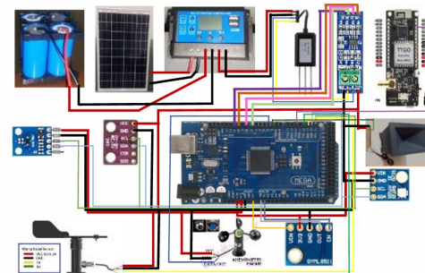
Gambar 15. Hardware design or wiring system on the AWS system
