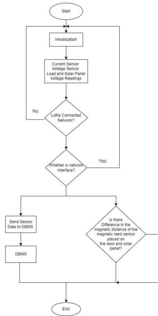
Gambar 4. Flowchart Hardware System Power Supply
