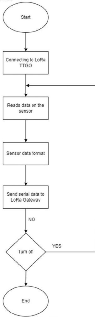
Gambar 1. Flowchart Node Sensor AWS
