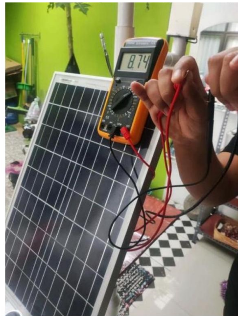
Gambar 6. Solar Panel Testing
