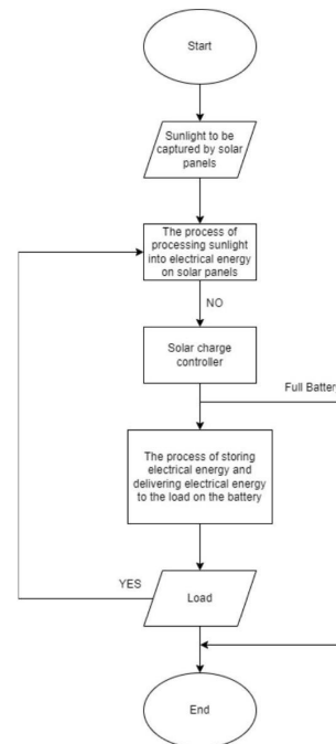
Gambar 3. Flowchart Hardware System Power Supply
