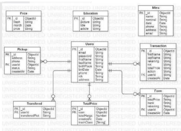
Gambar 1. Entity Relationship Diagram.
