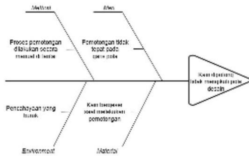
Gambar 2. Diagram Fishbone
